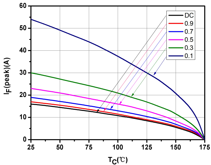
Fig.7-Current Derating
